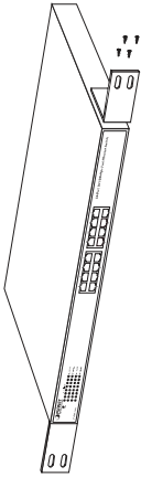
Figure 4: Attach the brackets to the Fast Ethernet Switch
